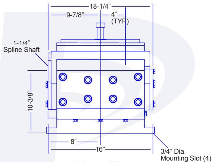
Fluid End View Hydraulic Drive Version
