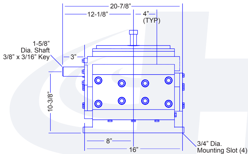
Fluid End View Shaft Drive Version
